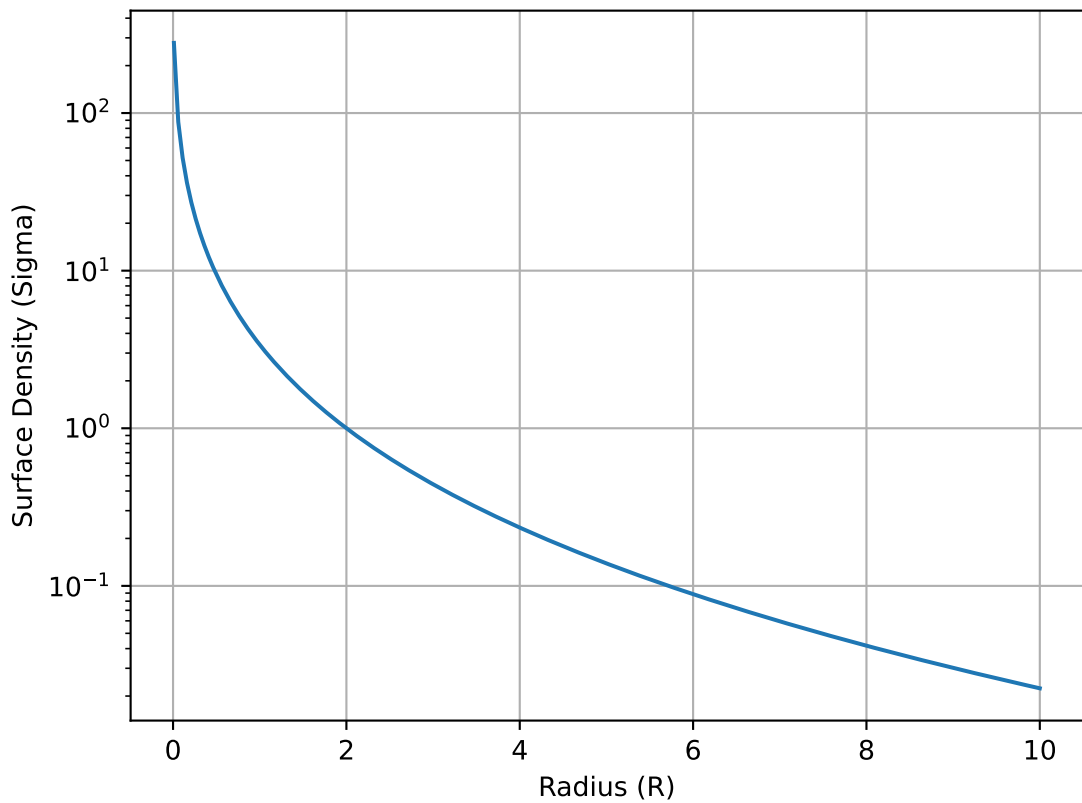
Sérsic Surface Profile (n=4)
