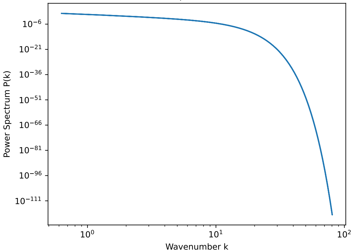
ZuHone+11 Spectrum with Cutoffs
