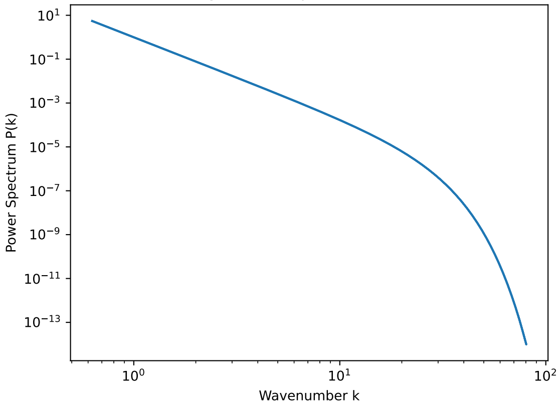
Kolmogorov-like Spectrum with Cutoff
