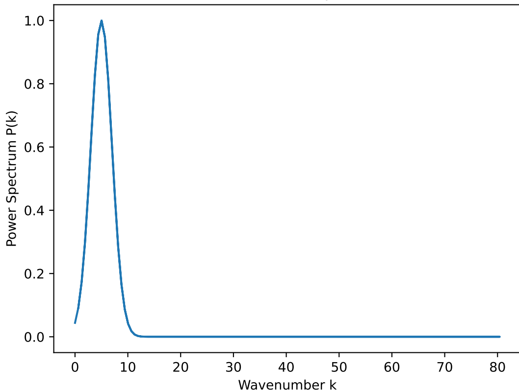
Gaussian-Cutoff Spectrum
