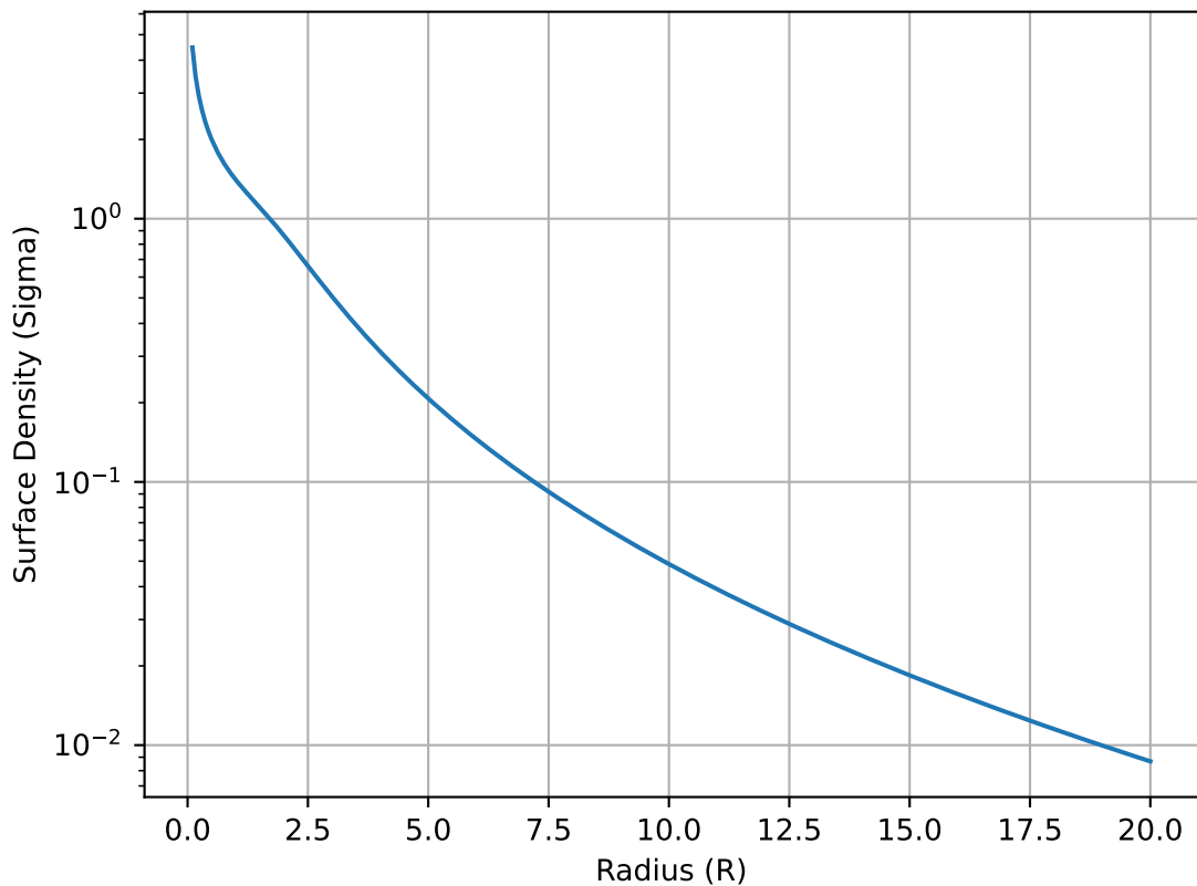
Core-Sérsic Surface Profile
