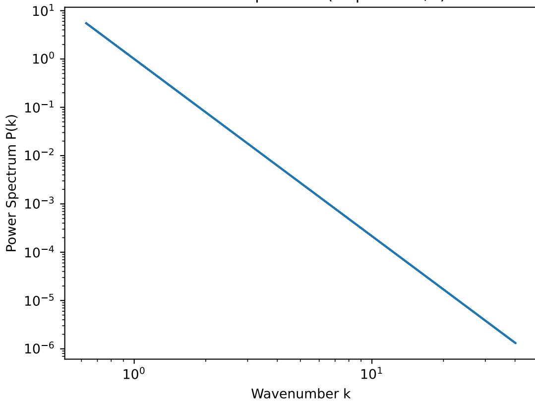
Power-Law Spectrum (slope = -11/3 )
